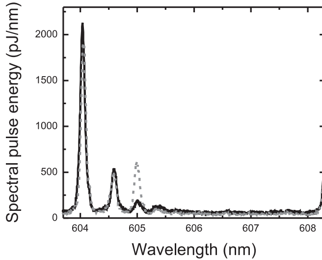
Figure 10.1: Two emission spectra of the random laser collected at the same spot on the sample. One spectrum (black solid line) before, and one (gray dashed line) after shifting the sample by 37\text{ }\mu\text{m} and back. Apparently, the frequencies of the modes are fully determined by the realization of the disorder.
