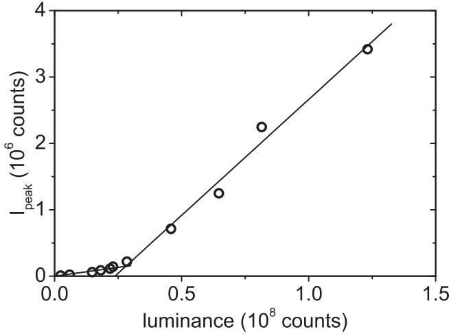
Figure 4.2: Measured integrated intensity in the \text{TE}_{95} mode versus luminance of a sphere with gain (the lines are a guide to the eye). The laser threshold is clearly visible.
