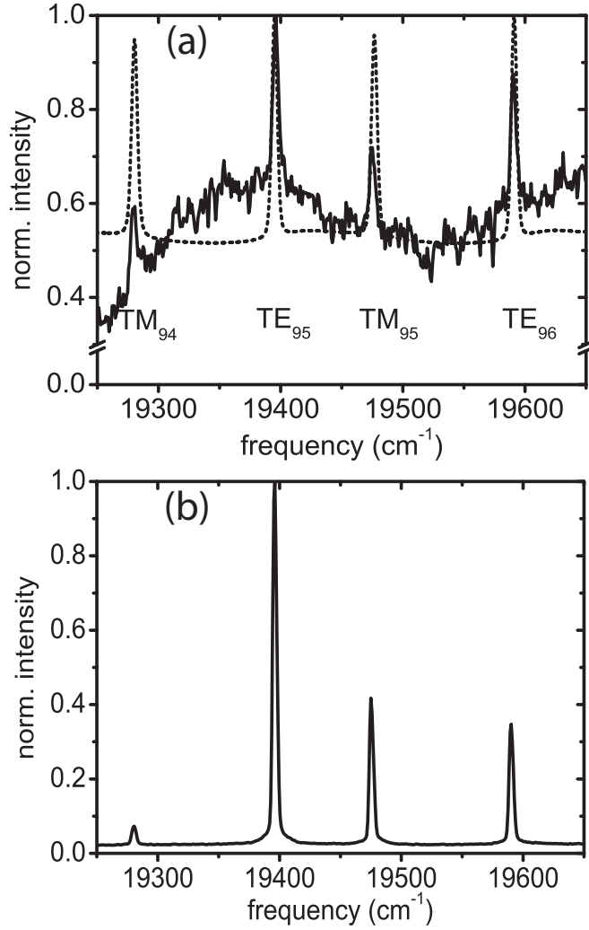
Figure 4.1: (a) Experimental emission spectrum of a microsphere excited with a low pumping power of 1 nJ/pulse (normalized to the peak intensity of the TE 95 mode). The dashed curve shows a theoretical fit of Mie theory. (b) Experimental spectrum of the same sphere measured at 100 nJ/pulse, above threshold.
