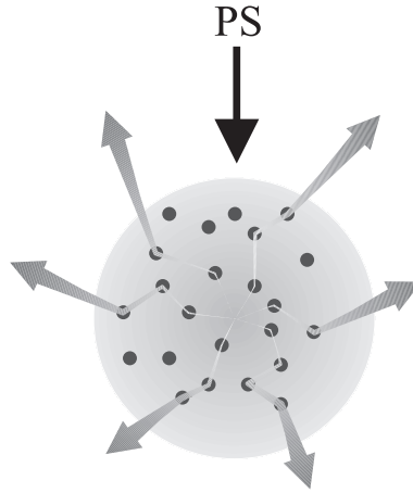
Figure 1.4: Schematical impression of a random laser: a gain medium (gray area) with randomly placed scatterers. The gain medium is pumped with an external pump source (PS). The resulting laser light is omnidirectional. (Figure taken from [83].)
