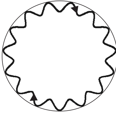
Figure 1.3: Schematical impression of a whispering gallery mode inside a microsphere. Light propagates along the boundary of the sphere, and interferes constructively after one round trip. If the whispering gallery mode is above its threshold, the intensity in that mode increases after each round trip.
