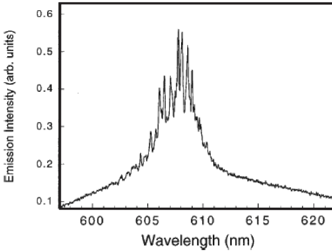
Figure 5.2: Measured emission spectrum of a random laser. Clearly visible are the narrow spectral features on top of the narrowed spectrum, referred to as spikes. (Figure taken from [26].)
